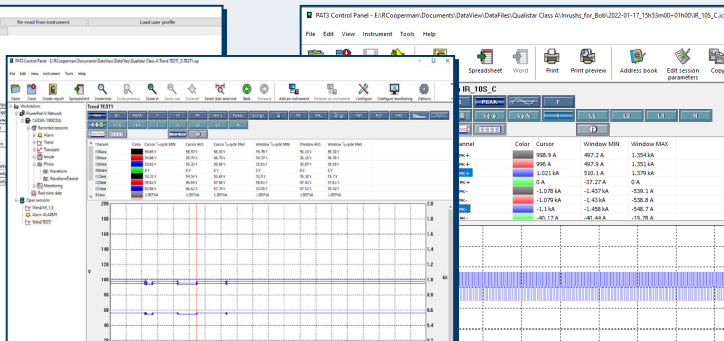
Display InRush peak.
